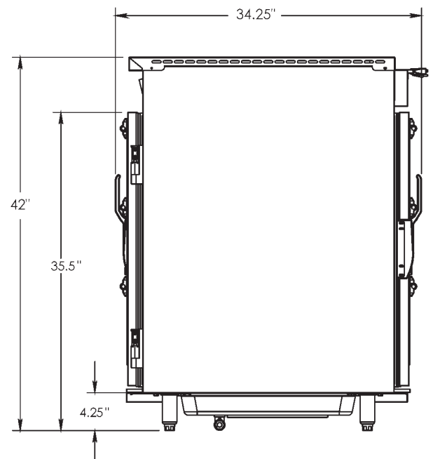
PHTT-6P-KFC Side View
