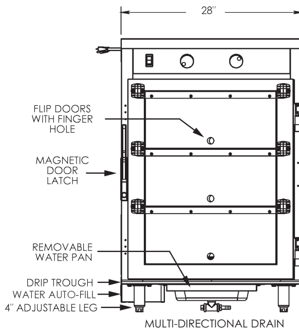
PHTT-6P-KFC Front View
