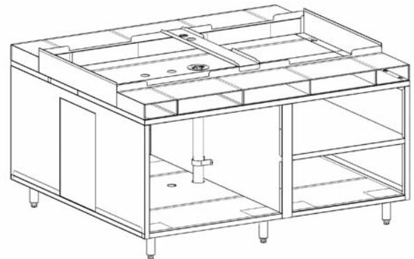
Isometric View of Assembled Components
