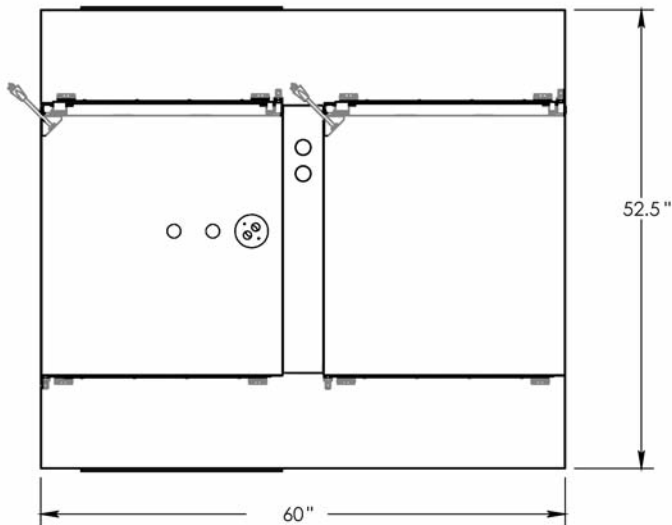
Top View With PHTT-5P-KFC or PHTT-6P-KFC Units in Place
